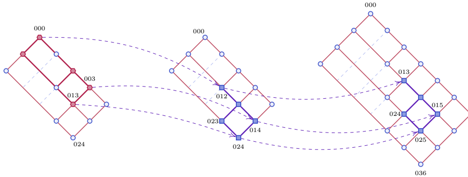
Figure 2.8: From the top to bottom and left to right, here are the posets \text{Ca}_2(3) , \text{Ca}_2(3) , and \text{Ca}_3(3) . The two last posets contain \mathcal{I}(\text{Hi}_1)(3) as subposets. There is a poset morphism between the output-wings of the first one and the input-wings of the second one.
