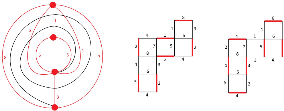
Figure 6.1: On the left is an arc \tau (black) and a triangulation T of an annulus. On the right are two matchings of the snake graph G_{T,\gamma} . The midpoint of the weight vectors of these matchings does not correspond to a matching.
