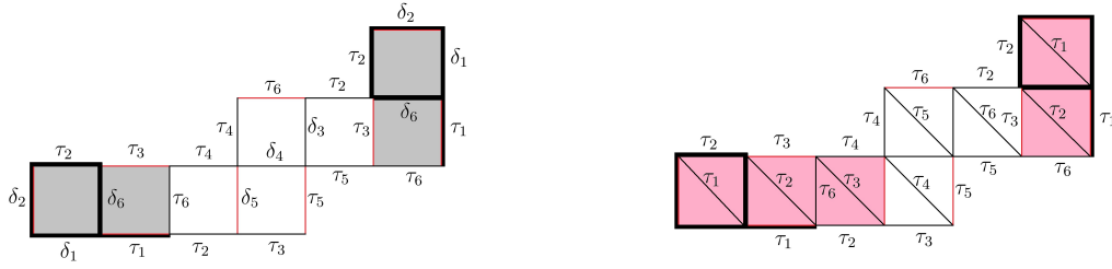
Figure 2.8: A \rho -symmetric matching M (red) of snake graph G_{T,\lambda} from Figure 2.7 with boundary frozen variables, and of the corresponding snake graph with principal coefficients. The pink squares correspond to C(M) . The edges of M are labeled, in counter-clockwise order starting from the bottom-left end: \delta_2, \tau_1, \delta_5, \tau_5, \tau_3, \tau_1, \delta_2, \tau_6, \tau_3 .
