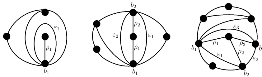
Figure 5.3: Examples of our notation for triangulations of punctured polygons with k = 1 , k = 2 , and k = 3 radii.
