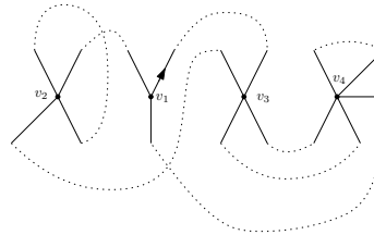
Figure 2.4: The map configuration model for \mathbf{d} = (3, 4, 4, 5) .
