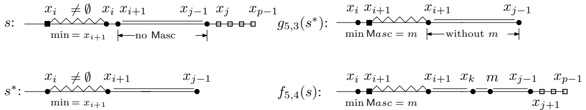
Figure 8.11: The construction of s \mapsto f_{5,4}(s) for Case 1 when the first Masc after the rightmost x_i is a right-to-left minimum. Here x_i = \text{Rmin}(s)_i , i = \text{rpos}(s) and \text{rmin}(s) = p .
