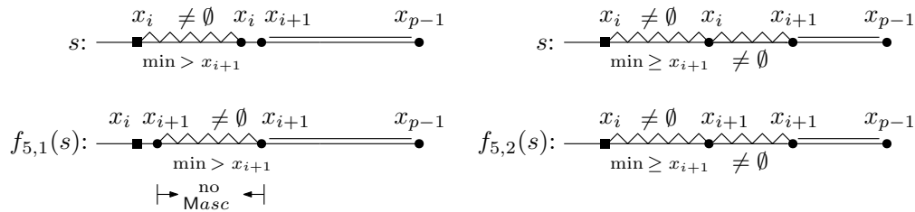
Figure 8.2: The bijections f_{5,1} and f_{5,2} in Lemma 8.2 and 8.3. Here x_i = \text{Rmin}(s)_i and i = \text{rpos}(s) .
