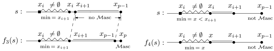
Figure 4.1: Two bijections f_3 and f_4 on ascent sequences s \in \mathcal{T}_3 \dot{\cup} \mathcal{T}_4 with \text{rpos}(s) = i and \text{rmin}(s) = p . Here x_i always denotes the entry of the i -th right-to-left minimum, so x_{p-1} is the last entry of s .
