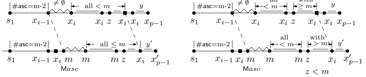
Figure 8.9: Case 4: the rightmost x_{i-1} is not next to x_i and the two rightmost x_i 's are next to each other. Here x_i = \text{Rmin}(s)_i with i = \text{rpos}(s) , z < m and y' = y + 1 if y \geq m ; otherwise y' = y .
