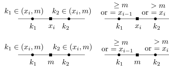
Figure 8.3: Substitution (1) in rule \mathcal{R}_1 . Here x_i = \text{Rmin}(s)_i and i = \text{rpos}(s) .
