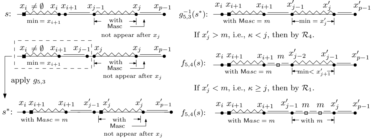
Figure 8.12: The construction s \mapsto f_{5,4}(s) for Case 2. Here \text{rmin}(s) = p , x_i = \text{Rmin}(s)_i with i = \text{rpos}(s) and y' = y + 1 if y \geq m ; otherwise y = y' .
