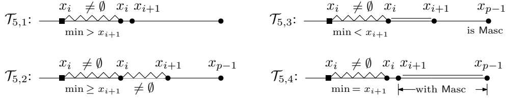
Figure 8.1: A partition of the set \mathcal{T}_5 : For any s \in \mathcal{T}_5 with \text{rpos}(s) = i and \text{rmin}(s) = p , x_i = \text{Rmin}(s)_i denotes the i -th right-to-left minimum of s ; black dots and squares represent the rightmost and the second rightmost entry respectively.
