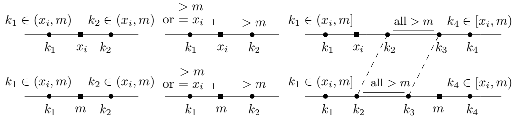
Figure 8.5: Substitution (5) and (6) in rule \mathcal{R}_2 . Here x_i = \text{Rmin}(s)_i with i = \text{rpos}(s) .
