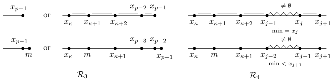
Figure 8.10: The insertion rules \mathcal{R}_3 and \mathcal{R}_4 where x_i = \text{Rmin}(s)_i , \text{rmin}(s) = p , \text{rpos}(s) = j and \kappa is the maximal index such that x_\kappa \leq m - 1 .
