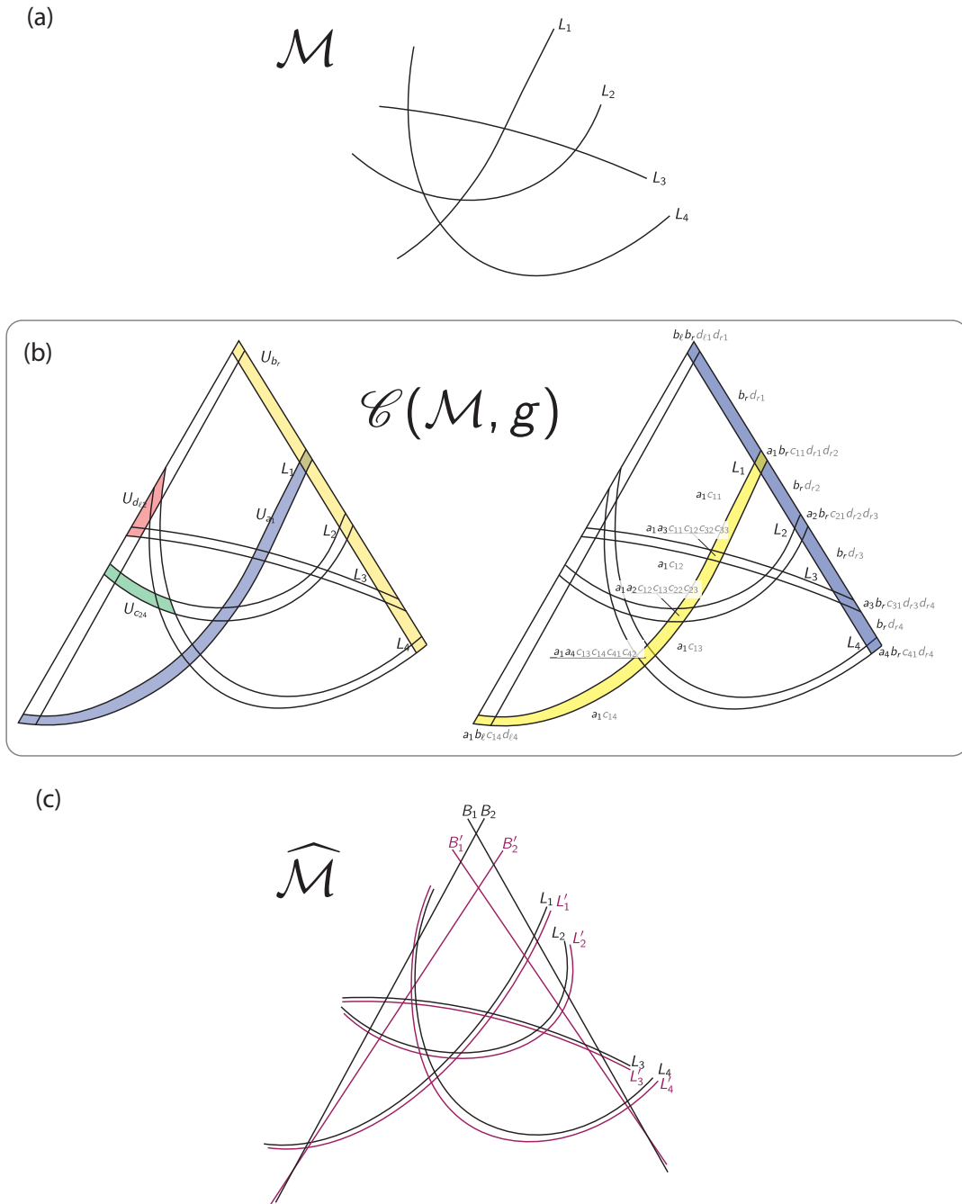
Figure 4.3: (a) A pseudoline arrangement for the oriented matroid \mathcal{M} . (b) A good-cover realization of the code \mathcal{C}(\mathcal{M}, g) . Left, representative open sets are shown. Right, select codewords are labeled. (c) A pseudoline arrangement for \widehat{\mathcal{M}} .
