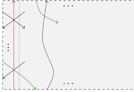
Figure 4.4: The red strand runs parallel to the left side of R , i.e., there are no triple crossings strictly between the red strand and the left side of R .
