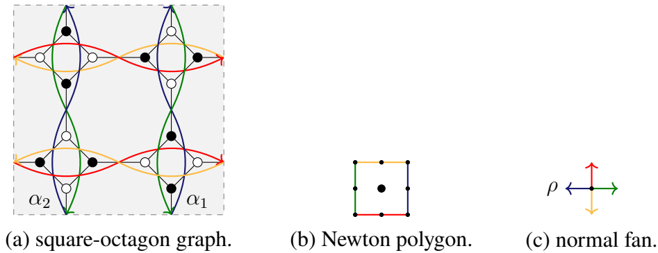
Figure 1.2: A square-octagon graph, its four-sided Newton polygon, and normal rays. For the blue ray labeled \rho , the set Z_\rho = \{\alpha_1, \alpha_2\} consists of the two blue zig-zag paths, and they are indexed so that the index increases along \rho (cyclically).
