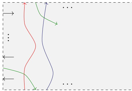
Figure 4.3: The configuration at the end of Step 1. There are no other endpoints of strands between the endpoints of \alpha_1 and the black strands (resp., between the endpoints of \alpha_2 and the black strands).
