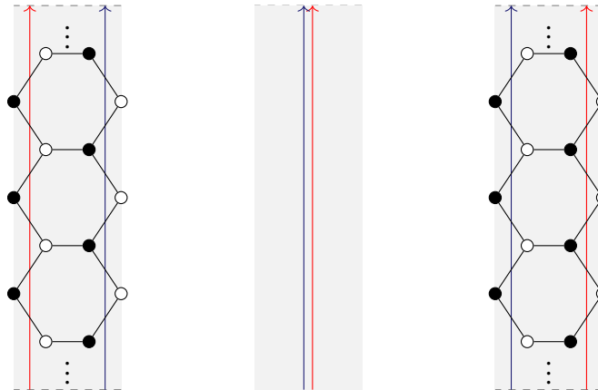
Figure 1.3: The geometric R -matrix transformation and the homotopy of zig-zag paths. The red and blue zig-zag paths on either side of the cyclic chain of hexagons interchange positions, whereas all other zig-zag paths are left unchanged.
