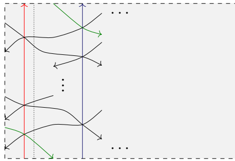
Figure 4.5: The blue strand runs parallel to the left side of R' , i.e., there are no triple crossings strictly between the red strand and the blue strand.
