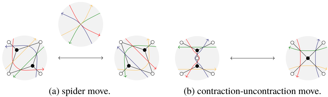
Figure 1.1: The elementary transformations, along with the corresponding homotopies of zig-zag paths. For the contraction-uncontraction move, the degree-two vertex getting contracted/uncontracted can be either black or white, and the two vertices adjacent to it are distinct and of degree at least two (here (b) illustrates the case when both degrees are equal to three).
