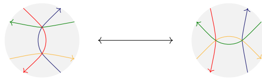
Figure 4.1: The 2 – 2 move.
