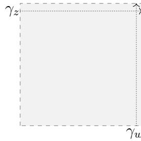
Figure 2.1: The fundamental rectangle R , along with the cycles \gamma_z, \gamma_w .
