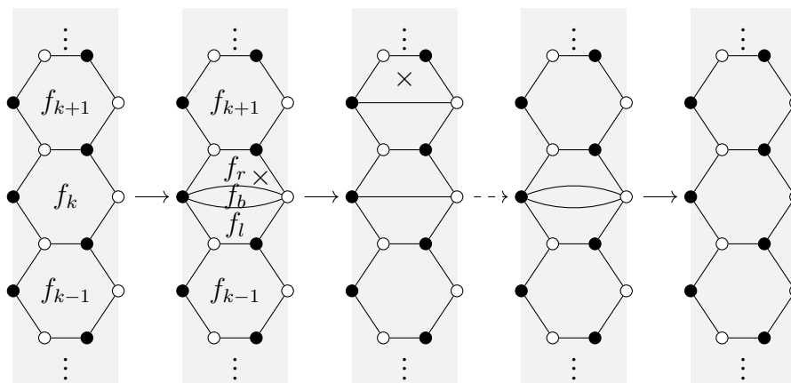
Figure 3.1: The sequence of moves in the geometric R -matrix transformation. The faces where we perform spider moves are marked by \times 's. The dashed arrow indicates a sequence of n - 1 spider moves.
