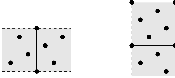
Figure 3.1: The strips of Lemma 3.2.
