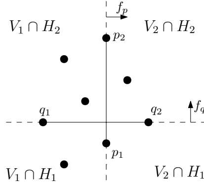
Figure 4.1: Setup for the proof of Lemma 3.2.
