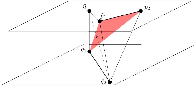
Figure 3.2: [\tilde{u}, \tilde{q}_2] intersects \text{conv}(\tilde{p}_1, \tilde{p}_2, \tilde{q}_1) .
