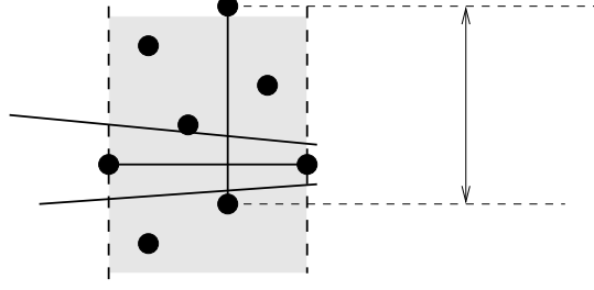
Figure 4.2: Illustration of the proof of Claim 4.2.
