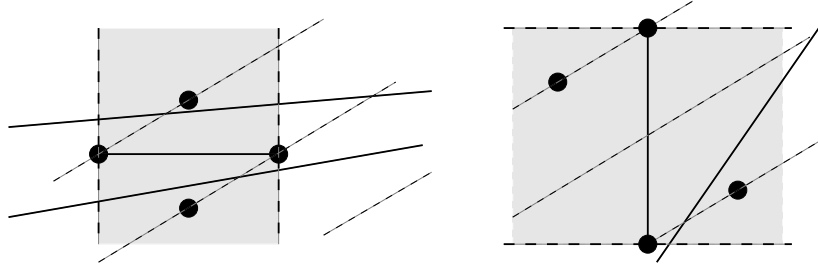
Figure 4.4: Illustration of the proof of Claim 4.4. The functional g is constant along the dashed diagonal lines.
