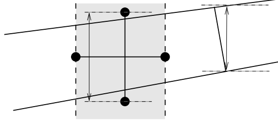
Figure 4.3: Illustration of the proof of Claim 4.3.
