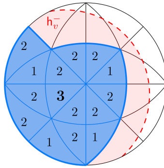
Figure 0.1: A sharp arrangement in \mathbb{R}^3 .
