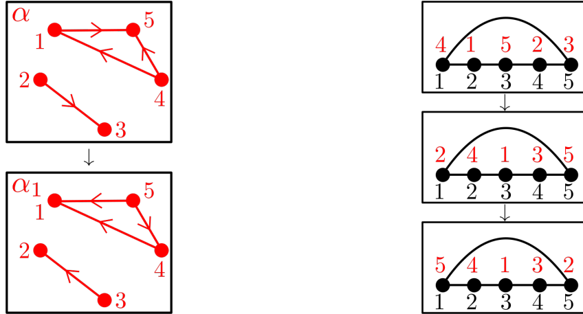
(a) Acyclic orientations \alpha, \alpha_1 \in \text{Acyc}(\overline{Y}) .
