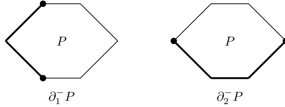
Figure 6.1: Visualizations of \partial_1^- P and \partial_2^- P when P is the hexagon with vertices \pm(2, 0), \pm(1, 1), \pm(1, -1) . Thick lines correspond to \partial_1^- P and \partial_2^- P .
