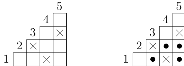
Figure 7.2: Left: rook placement for \mathcal{A} = 14|235 . Right: \rho(P) = 3 .
