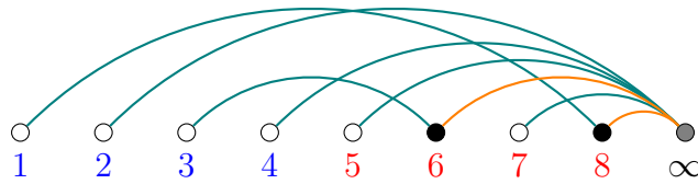
Figure 3.3: Extended chord diagram for \mathcal{A} = 18|2|36|4|5|7 . First arcs and second arcs are colored differently. When \alpha = (4, 4) , \alpha -interlacings are given by \{(3, 6), (4, \infty)\} , \{(1, 8), (2, \infty)\} and \{(1, 8), (4, \infty)\} . Thus i_\alpha(\mathcal{A}) = 3 .
