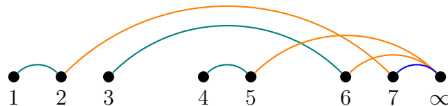
Figure 3.1: Extended chord diagram of the partition 127|36|45 . The j th arcs in each block are colored identically for j \geq 1 .
