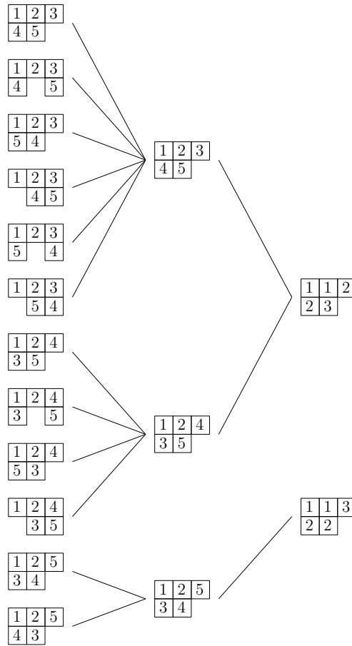
Figure 2.3: The set partitions, tableaux and semistandard tableaux corresponding to the maps \mathcal{T} and \mathcal{S}_\alpha for \mu = (3, 2) and \alpha = (2, 2, 1) .
