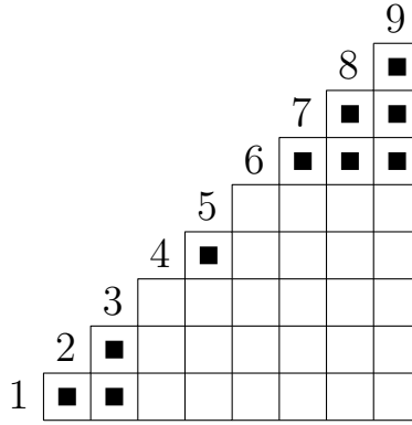
Figure 7.3: The forbidden squares for rooks when \nu = (3, 2, 4) .
