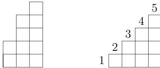
Figure 7.1: Left: the Ferrers board B(2, 4, 5) ; Right: the staircase board of size 5 with rows and columns labeled.
