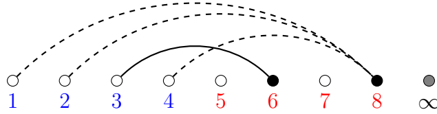
Figure 3.2: Choices for \theta(8) when \theta(6) = 3 . Numbers of the same color are in the same block of \mathcal{A}_\alpha . White and black nodes correspond to elements in the first and second row of the tableau respectively.
