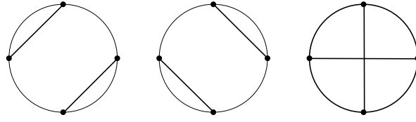
Figure 5.1: All chord diagrams on 4 points.
