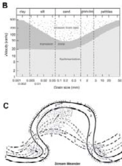
Figure 14b Velocity of fluids is an important factor in moving grains. Velocity can also affect river bottoms and cause erosion.
