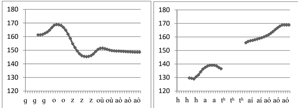
Figure 9. Locative inflection and tone spreading. Averaged time normalized pitch contour for the nouns gozouàò ‘water-Loc’ and hat h aiáó ‘house-Loc’ (n=25)
