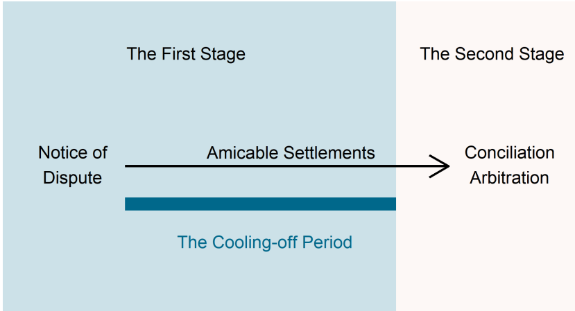
Figure 1. ISDS Timeline
