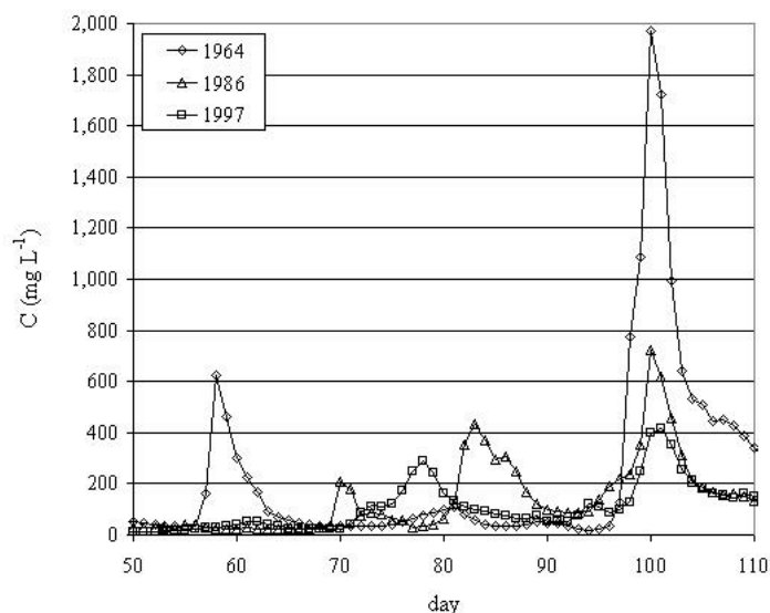
Figure 12. Daily concentration (C) on the Sacramento River upstream from the Yolo Bypass for the floods of 1964, 1986, and 1997.
