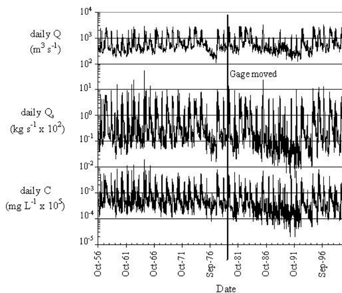
Figure 3. Daily flow ( Q ), suspended-sediment discharge ( Q_s ), and concentration ( C ) for the Sacramento River at Sacramento/Freeport. Note that Q_s and C were scaled to separate the records vertically.
