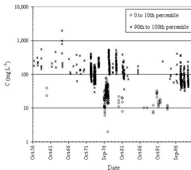
Figure 9. Individual concentration measurements for the 0 to 10th and 90th to 100th percentile ranges of flow, Sacramento River at Sacramento/Freeport.
