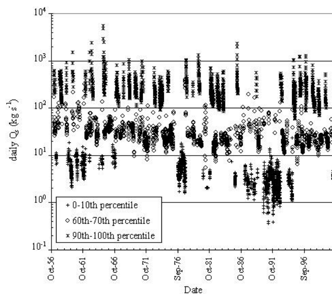
Figure 8. Daily suspended-sediment discharge ( Q_s ) for the 0 to 10th, 60th to 70th, and 90th to 100th percentile ranges of flow, Sacramento River at Sacramento/Freeport.
