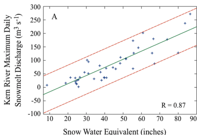
Figure 23. An example correlation of annual maximum daily snowmelt discharge amplitude with annual initial snow water equivalent, Kern River at Kernville. The red lines are plus and minus two standard deviations from the correlation.
