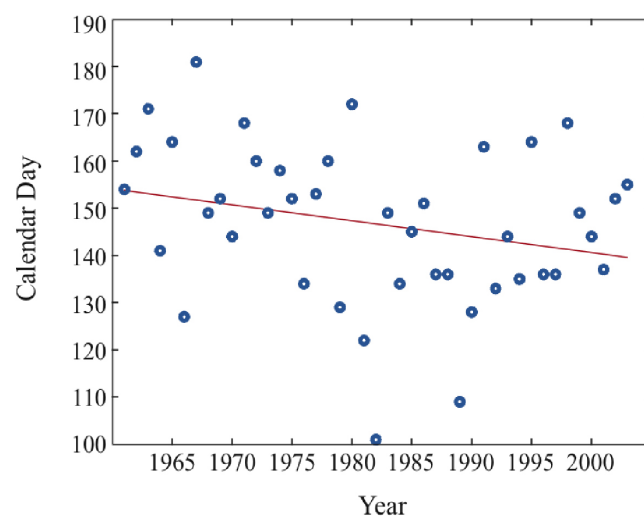
Figure 11. Trend in the timing of snowmelt discharge based on the day of maximum daily discharge (peak flow), Kern River.
