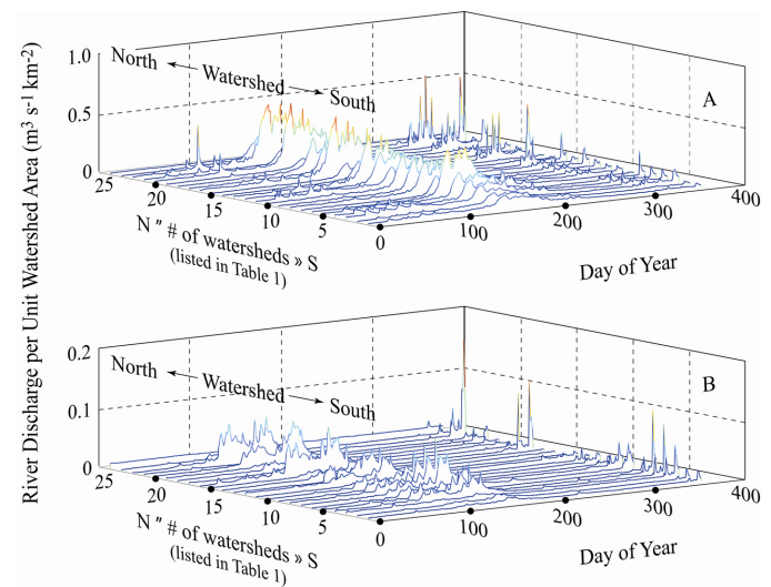
Figure 6. Daily south-to-north Sierra Nevada snowmelt runoff (discharge normalized to the watershed area above the river discharge gage) in a wet year, 1983 (panel A), and in a dry year, 1977 (panel B). The south-to-north increase in runoff is especially distinct in the wet year. Also the difference in runoff between the wet and dry years is almost an order-of-magnitude (the vertical scales change between A and B). Note the sharp winter rain-derived river discharge peaks near the end of the wet and dry years. In these two ENSO years, the relative amount of rain appears to increase from south to north in the wet year (upper graph) and appears uniform in the dry year (lower graph).
