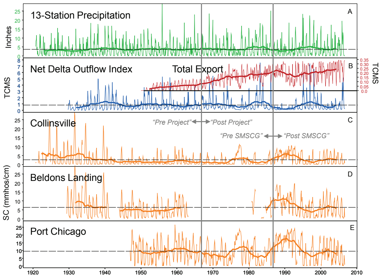
Figure 2 (A): Monthly average of 13 Sierra Nevada foothill precipitation stations on tributaries of the San Francisco Estuary watershed (1920-2006). (B): Monthly Delta outflow index. Right axis is monthly average total water project export. (C,D,E): Monthly average specific conductivity for Collinsville, Beldons Landing, and Port Chicago. Prior to 1966, SC is estimated from approximately four high tide TDS grab samples per week. Heavy solid line is 5-year running average. Dotted line is period of record mean.
