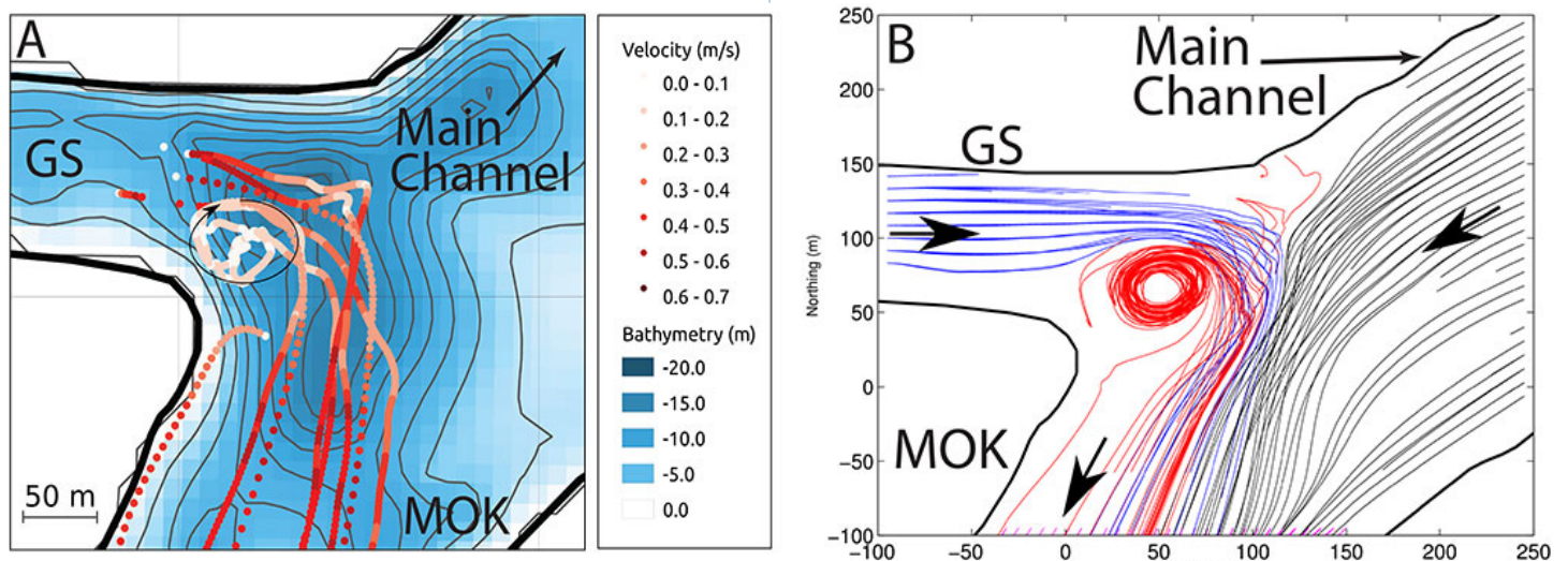
Figure 9 Drifter paths (A) and SUNTANS streamlines (B) reveal a recirculation zone at the west junction (GS/MOK). (A) Group 12 drifter paths on June 8, 2012, from 13:36 to 15:14 during the ebb tide. (B) SUNTANS streamlines on May 30, 2012 at 14:00 where red lines denote streamlines originating from the corner region, blue lines originate from GS, and thin black lines originate from the main channel to the northeast of GS.
