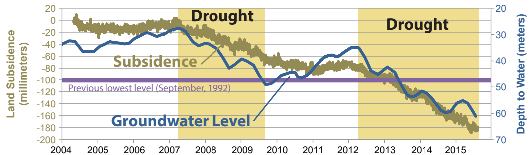
Figure 2 Graph showing vertical displacement at a selected GPS station and depth to water in a nearby well for 2004–2015 (see Figure 1 for location)
