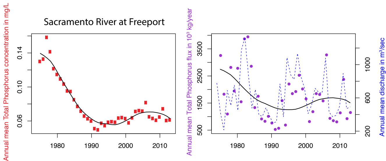
Figure 3 TP concentration and flux at the Sacramento River at Freeport site. Annual mean concentrations of TP (solid red dots), annualized total load of TP (purple dots), annual mean discharge (dashed blue line), and flow normalized trends (solid black lines) are shown.
