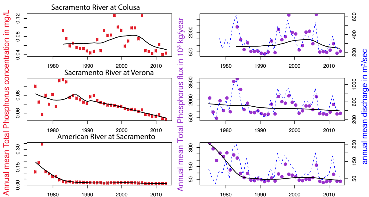
Figure 5 TP concentration and flux for three Sacramento River Basin sites. Annual mean concentrations of TP (solid red dots), annualized total load of TP (purple dots), annual mean discharge (dashed blue line), and flow normalized trends (solid black lines) are shown.
