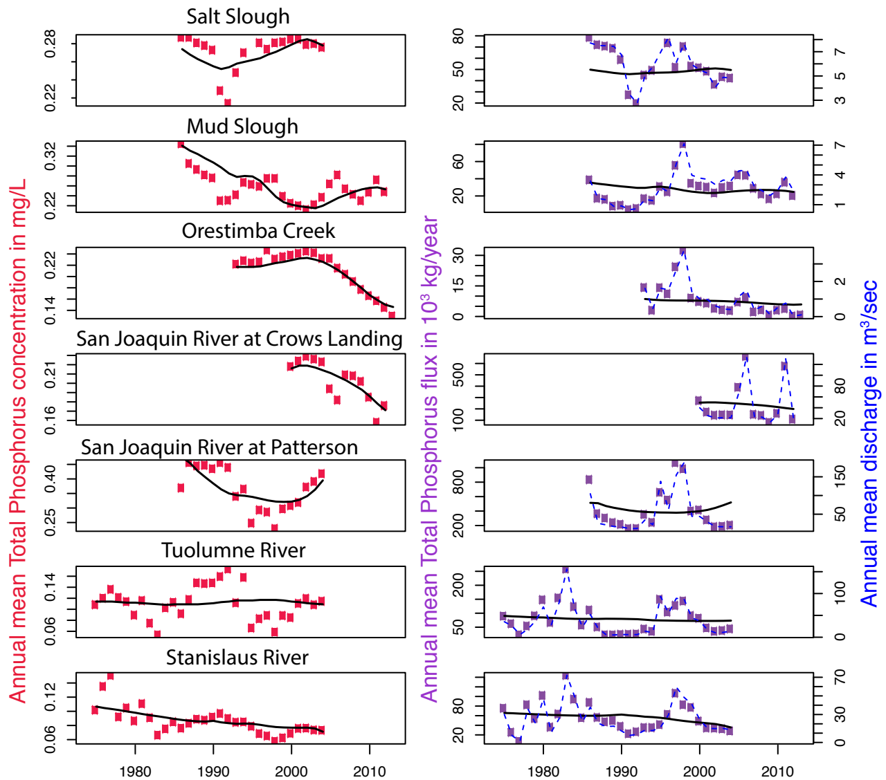
Figure 13 TP concentration and flux for seven San Joaquin River basin sites modeled. Annual mean concentrations of TP (solid red dots), annual total load of TP (purple dots), annual mean discharge (dashed blue line), and flow normalized trends (solid black lines) are shown.
