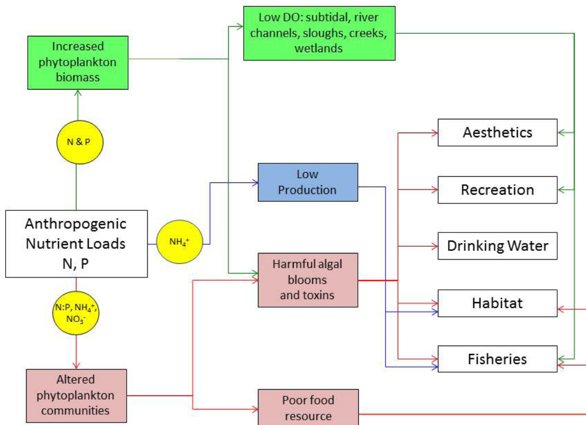
Figure 4 Conceptual model of potential pathways for nutrient-mediated ecosystem disruptions via phytoplankton processes in the high nutrient Delta (modified from Senn and Novick [2014a]). Green boxes represent pathways leading to the “classical” cultural eutrophication response. The blue box highlights the pathway described by the Ammonium Paradox (Dugdale et al. 2007), and red boxes highlight the pathways described by ecological stoichiometry theory (Glibert et al. 2011).
