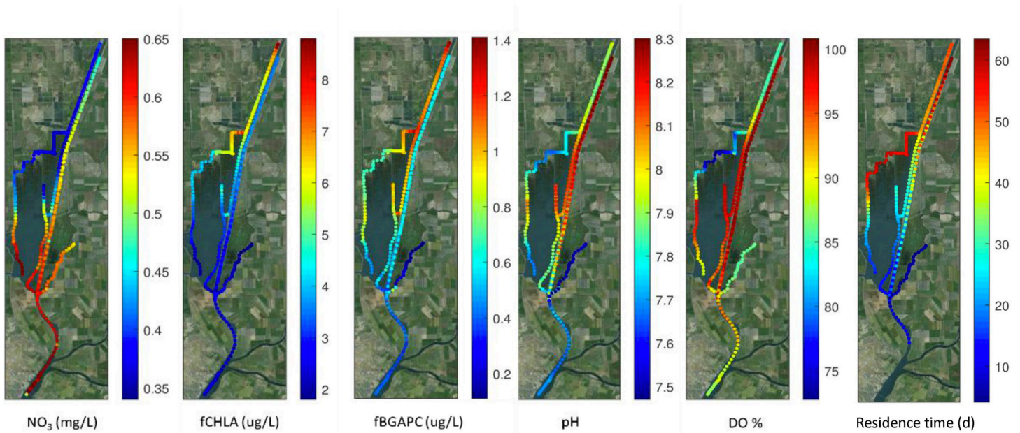
Figure 12 Concurrent high speed mapping of nitrate [ \text{NO}_3^- ], Chlorophyll fluorescence [fCHLA], Phycocyanin fluorescence [fBGAPC], pH, Dissolved oxygen [DO%] and water residence time (days) show how environmental gradients are related to residence time. Data were collected on October 1, 2014, over a period of approximately four hours starting at the flood to ebb transition.
