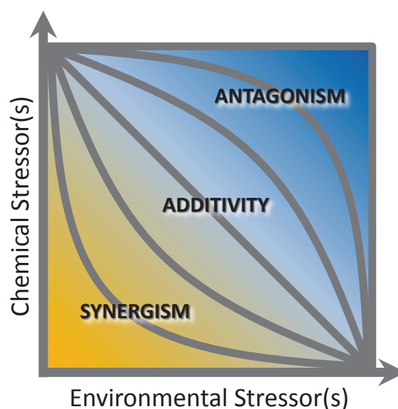
Figure 1 Isobologram depicting potential synergistic, additive and antagonistic effects resulting from the interaction of contaminants (e.g., pesticides) and environmental stressors (e.g., temperature). Highest values on the X and Y axes correspond to equivalent responses (e.g., equal percentage mortality) resulting from exposure to each respective stressors. These points are connected by lines that represent equal effect; isoboles , depicting their interaction.
