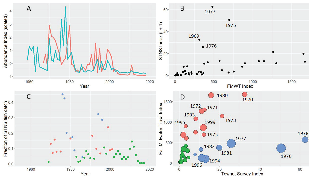
Figure 6 Population-dynamic plots for Delta Smelt: (A) z-scored time-series of the Summer Townet Survey (STNS; cyan) and Fall Midwater Trawl Survey (FMWT; orange) abundance indices. (B) Scatterplot of the FMWT versus subsequent-year STNS. Selected years are labeled, and reflect the year the FMWT sampling was conducted. The STNS is labeled t + 1 to denote that it is data collected from the calendar year that follows the FMWT. (C) Time-series of Delta Smelt’s fraction of the fish catch from the STNS for 1969–2015 (i.e., the years used to generate the bubble plot in panel D; 2016 and 2017 were unavailable when the database was downloaded, so these years were given the same near-zero fraction as 2015: 0.0047). (D) The STNS versus the next FMWT, which begins sampling 1 to 2 months after the STNS is finished. The data points sizes are scaled to Delta Smelt’s fraction of the total fish catch in the STNS (maximum = 0.45 per panel C). In panels C and D, higher survival years are colored orange, lower survival years are colored blue, and years in which survival cannot be visually characterized as higher or lower are colored green. Selected years of higher and lower survival are labeled in panel D.
