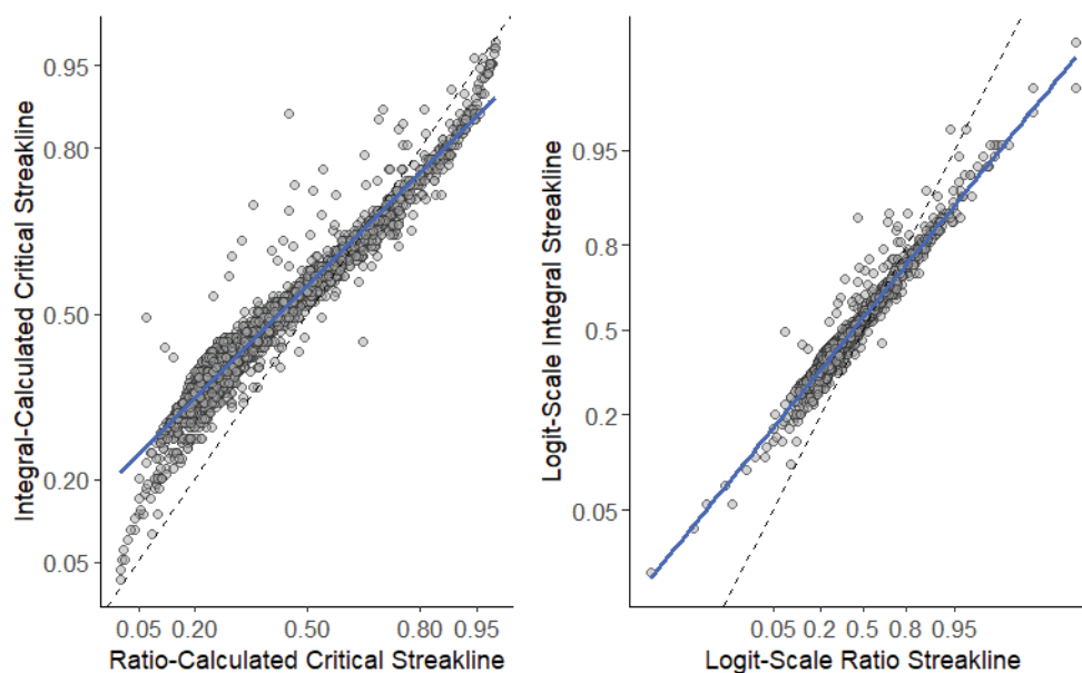
Figure 3 The location of the critical streakline calculated using two methods: the ratio of discharge between the junctions and the integration of velocity vectors on the normalized and the logit-scale. Under normalization, 0 indicates the left (SE) bank and 1 the right (NW) bank of the Sacramento River. The dashed line indicates the 1:1 line; the solid line represents the linear regression fit to the raw and transformed data. The non-linear shape of the untransformed data is a result of steepening of river bed slope near the banks.
