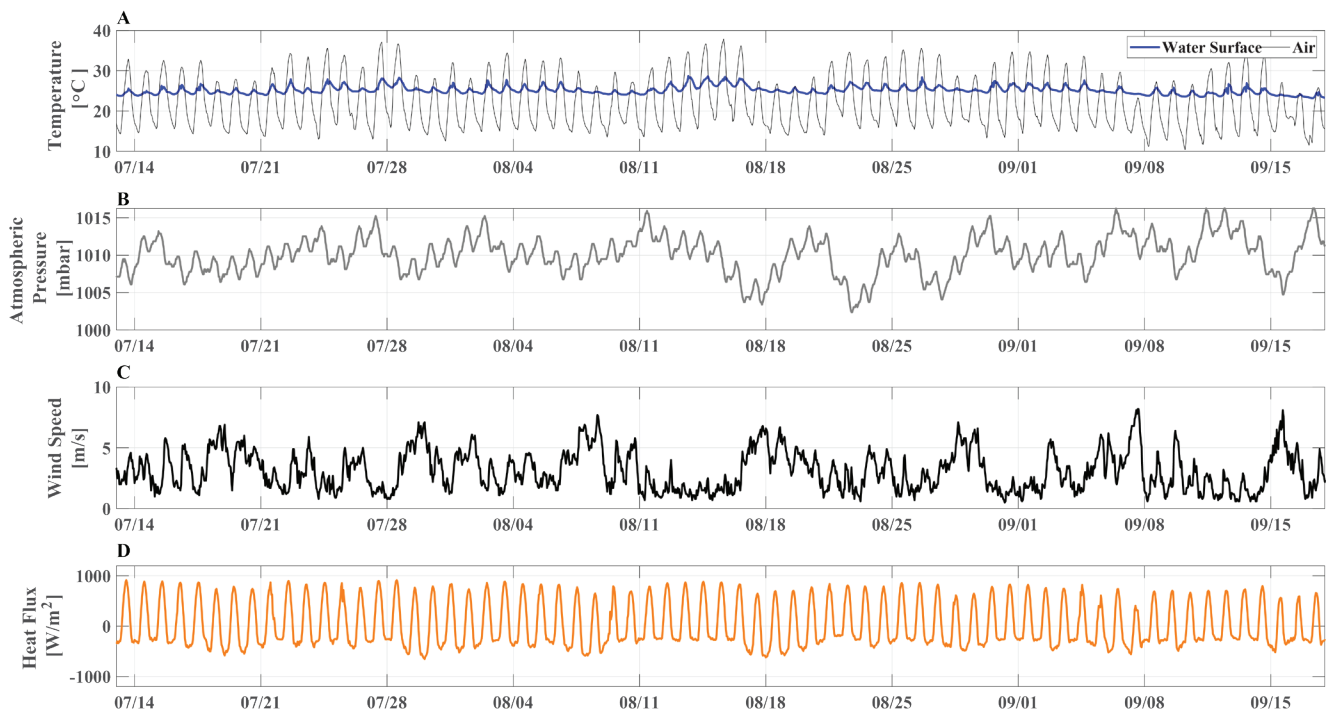
Figure 4 Components of the heat flux calculation (Equation 17): (A) water temperature (blue), air temperature (black), (B) atmospheric pressure, (C) wind speed, and (D) net heat flux. Meteorological data are from CIMIS station 121 in Dixon, CA.
