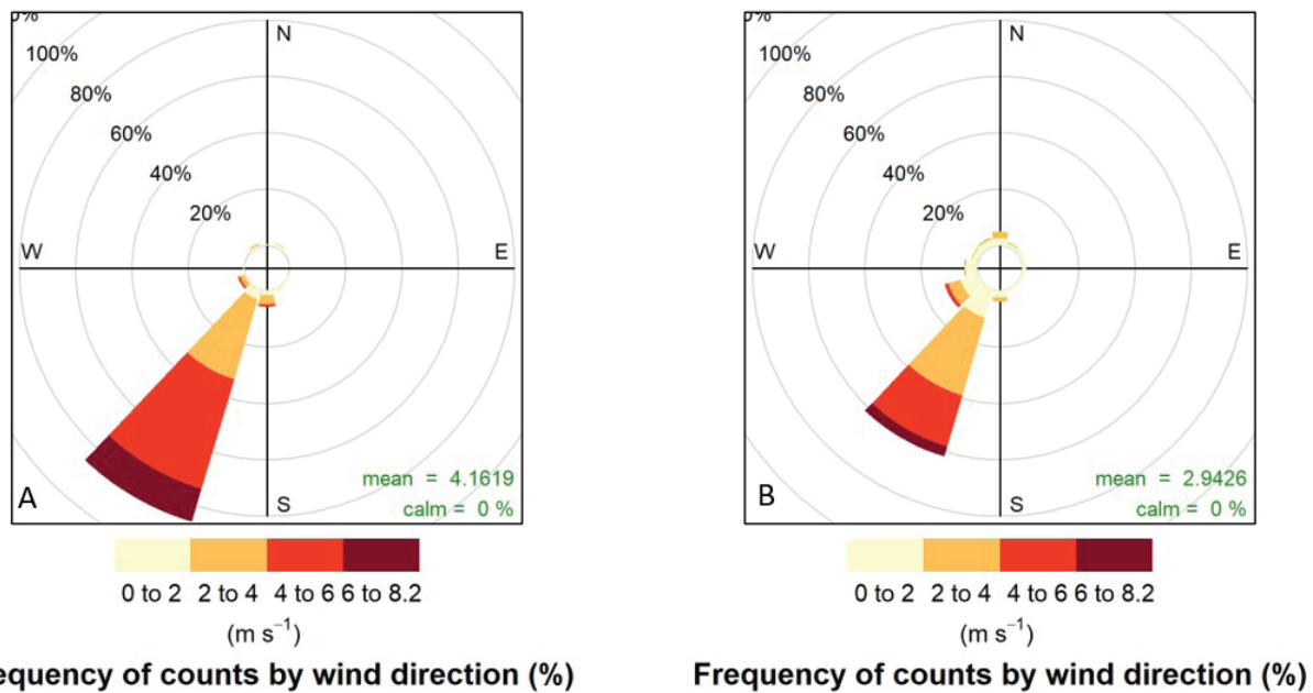
Figure 3 Wind rose summarizing hourly wind speed ( \text{m s}^{-1} ) and frequency of counts (%) by meteorological wind direction during (A) late afternoon and evening (16:00 to sunset) compared to (B) all other times of day over the experiment (7/2/19 to 9/18/19) from the Dixon weather station (CIMIS ID 121)
