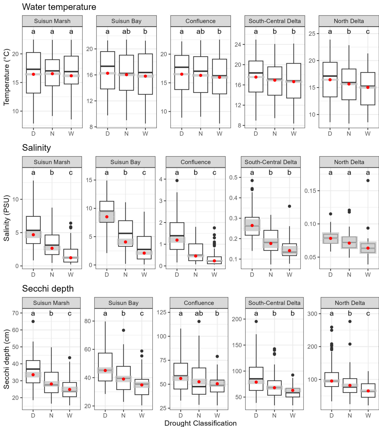
Figure 5 Observed values ( boxplots ) and model results (model means as red points \pm 95\% confidence intervals as gray boxes ) for the drought classification comparisons (drought period [D], neutral [N], and wet period [W]) by region for the water quality parameters. Different letters above boxplots identify statistically significant ( p < 0.05 ) differences from a Tukey post-hoc test.
