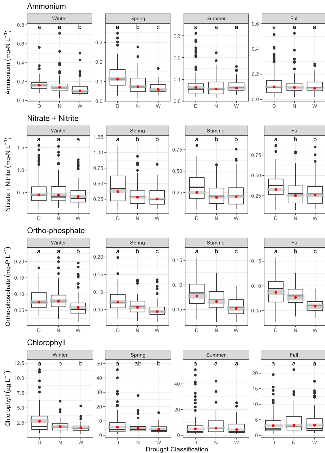
Figure 8 Observed values (boxplots) and model results (model means as red points \pm 95\% confidence intervals as gray boxes) for the drought classification comparisons (drought period [D], neutral period [N], and wet period [W]) by season for the nutrient and chlorophyll parameters. Different letters above boxplots identify statistically significant ( p < 0.05 ) differences from a Tukey post-hoc test.
