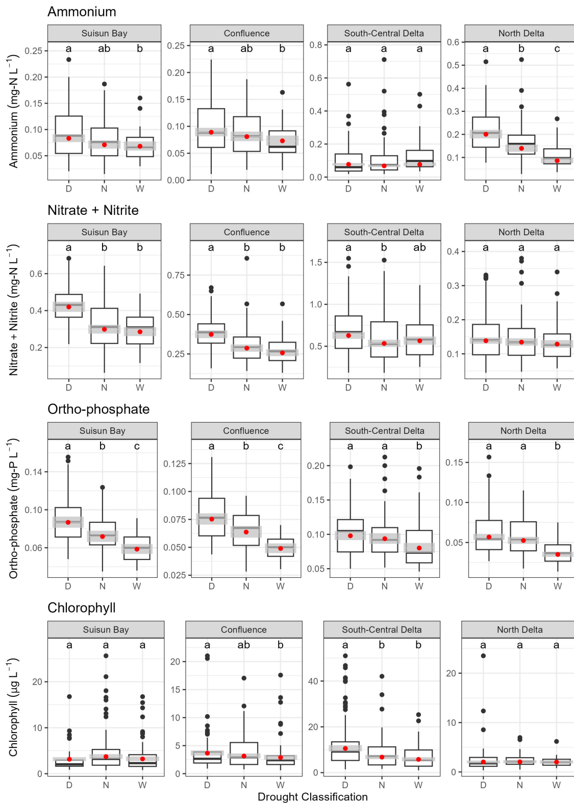
Figure 7 Observed values (boxplots) and model results (model means as red points \pm 95\% confidence intervals as gray boxes) for the drought classification comparisons (drought period [D], neutral period [N], and wet period [W]) by region for the nutrient and chlorophyll parameters. Different letters above boxplots identify statistically significant ( p < 0.05 ) differences from a Tukey post-hoc test.
