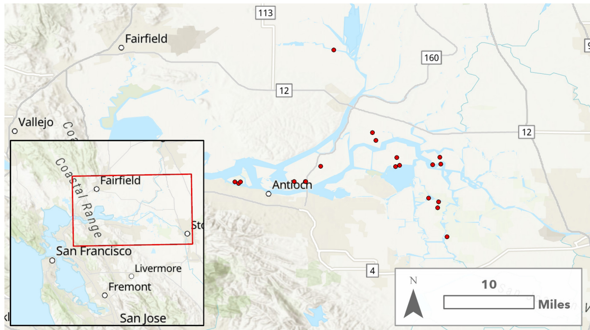
Figure 1 Sampling locations of peat cores used in peat core data synthesis
