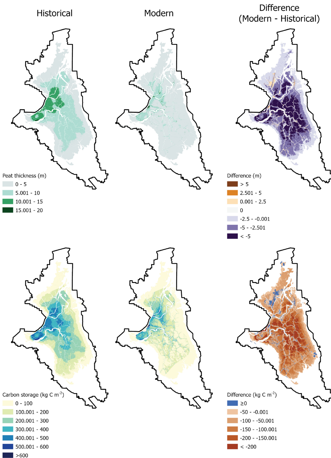
Figure 2 Mapped changes over time in peat thickness and peat carbon storage in the Sacramento-San Joaquin Delta. Historical maps illustrate modeled peat conditions in the early 1800s, and Modern maps depict estimated peat depths and carbon stocks in 2017. Mapped differences show changes in peat volume and carbon from oxidation and compaction, where negative values indicate a net loss over time of peat or peat carbon.
