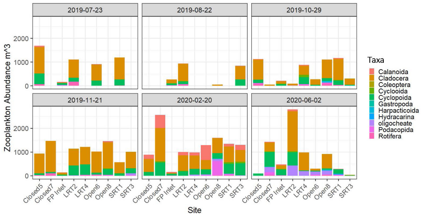
Figure 4 Stacked bar graphs of pelagic zooplankton abundance within the floating peat mesocosms for all quarterly sampling dates. SRT = short residence time, LRT = long residence time, Closed = full floating peat coverage, Open = half floating peat coverage, and FP Inlet = the adjacent South Fork Mokelumne River. Results for 2019-07-23 include only the pools that had peat blocks and received water. Closed7, LRT4, Open8, and SRT3 had yet to receive peat and be filled with water.
