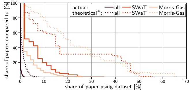
Figure 9: On average, authors compare IIDSs to 0.5 approaches from the related work (black), while theoretically, they could compare to at least 6.0. This gap increases for papers evaluating the SWaT or Morris-Gas datasets.
