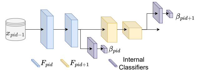
Figure 6: Internal Classifier Architecture: Each internal classifier allows requests to exit in the middle of an NN. For example, \beta_{pid} of requests exit at NN partition F_{pid} .
