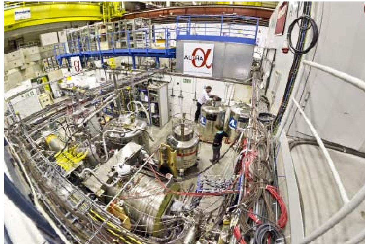
Figure 2. An external view of the ALPHA apparatus.
