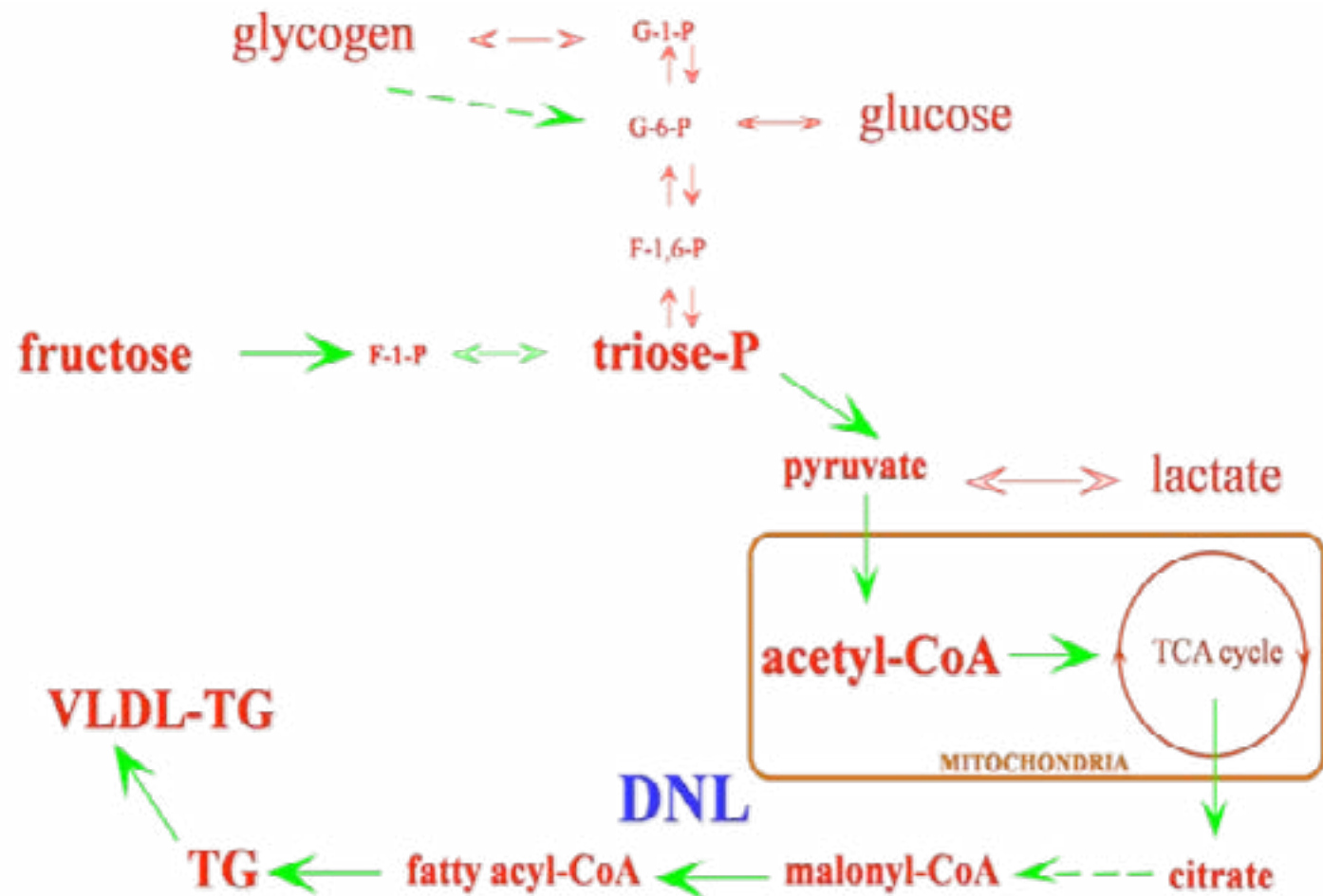
Figure 2. Metabolic pathways of fructose vs. glucose, leading up to de novo lipogenesis (DNL)
