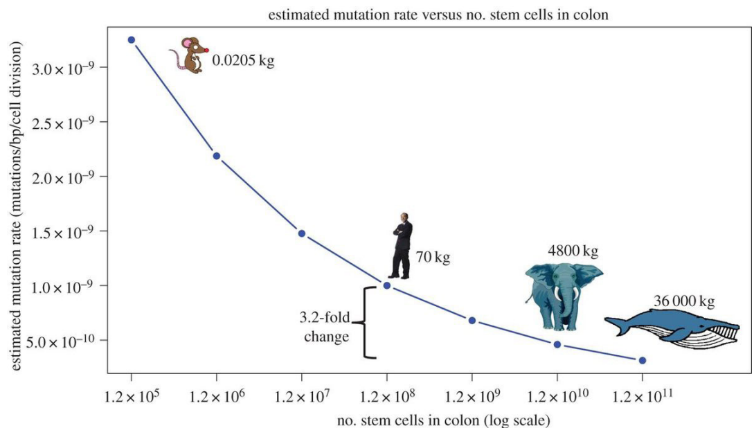
Figure 4: A graphic representation comparing mutation rates to the number of stem cells found in an animal. The number of stem cells found in an area allows researchers to project the total number of cells that an animal possesses. Notice how larger animals actually see less mutation in their cells than humans do, despite being considerably larger. Licensed under CC BY 4.0.
