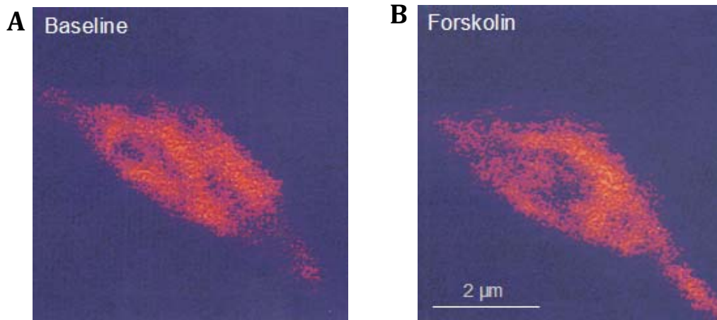
Figure 4: F-actin binding marker phalloidin conjugated to Alexa488 (15 \mu\text{M} in 200 mM KCl) showed A , baseline (drug-free) actin cytoskeleton arrangement in a presynaptic bouton. B , phalloidin-marked actin exhibits relocation and rearrangement in the same presynaptic bouton when perfused with adenylate cyclase activator forskolin (30 \mu\text{M} ).
