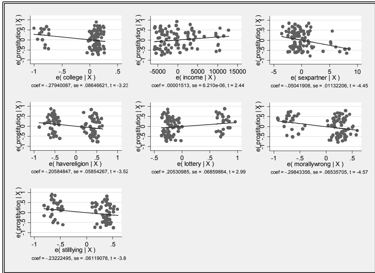
FIGURE 3 ADDED-VARIABLE PLOTS
