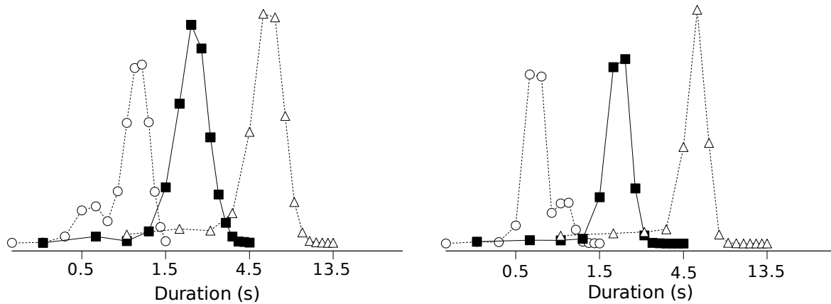
Figure 6. Simulation results of the LeT model. In each panel, the left, middle, and right curves show the density function of the intervals produced when the reinforced ranges were 0.5-1.5, 1.5-4.5, and 4.5-13.5, respectively. Left: \mu_\tau = 0.5 s, \sigma_\tau = 0.075 s, \beta = 0.02 , and \alpha = 0.16 . Right: \mu_\tau = 0.3 s, \sigma_\tau = 0.03 s, \beta = 0.04 , and \alpha = 0.20 .
