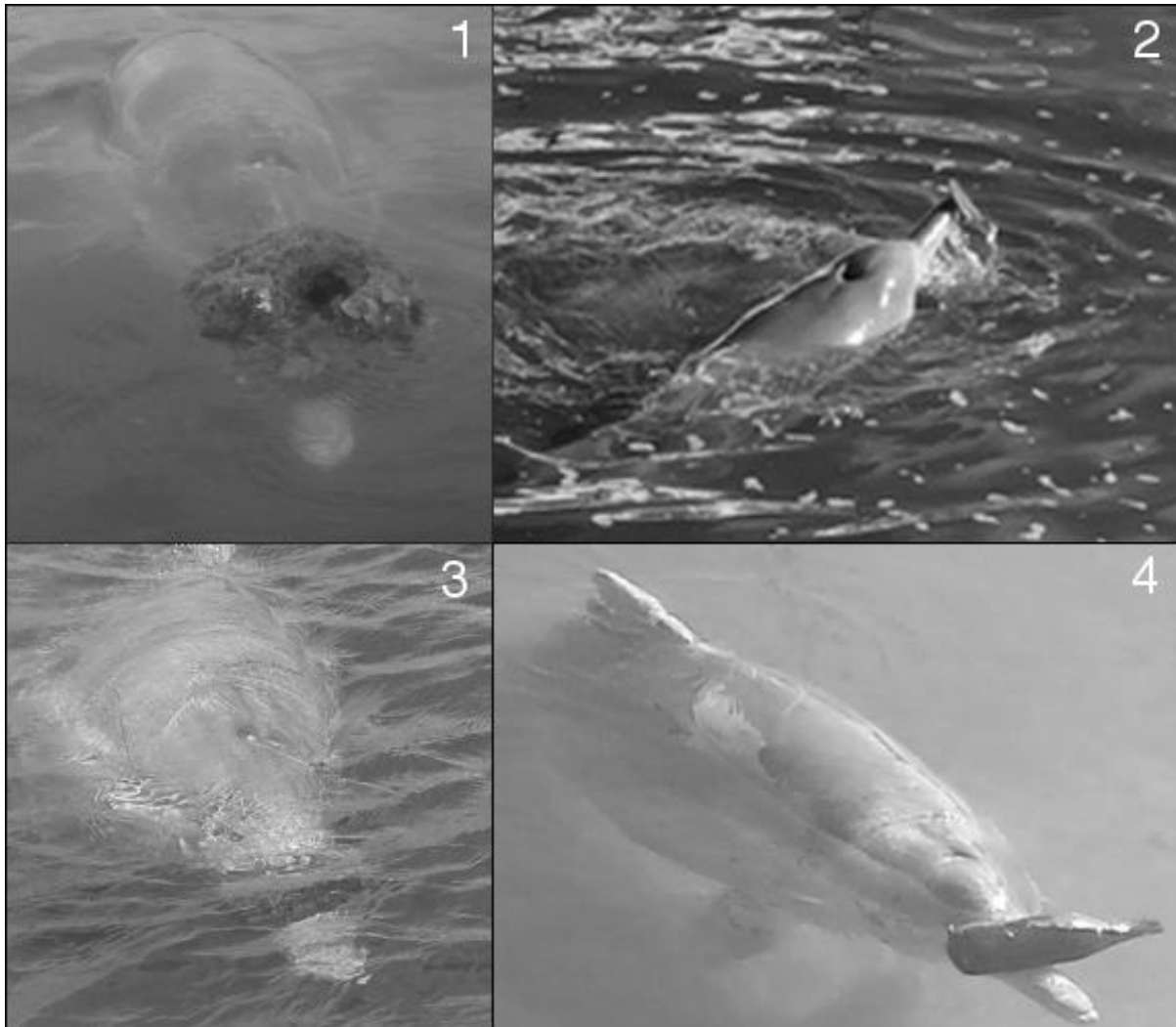
Figure 1. Study dolphins, adult and juvenile male Australian humpback dolphins, Sousa sahulensis , carrying 1. Sponge, 2. Leaf on tip of rostrum (juvenile), 3. Brick and 4. Bottle. (Photographs copyright 1. C. Austin; 2. T. Barber; 3. B. Lambert; 4. J. Smith.)
