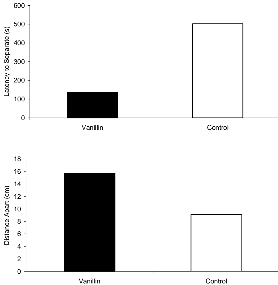
Figure 1. Latencies for pairs of chicks to move 20 cm apart and their social dispersal scores (mean distance apart) when tested in a novel environment in the presence or absence of a familiar odourant.
