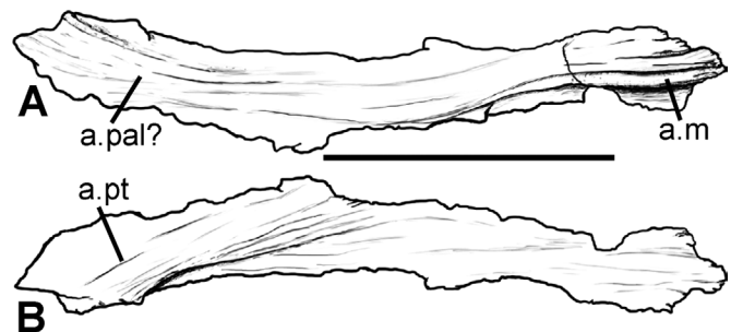
Figure 14. Postosuchus kirkpatricki (TTUP 9002) right vomer. A. Dorsal view. B. Ventral view. Scale bar = 5 cm.
