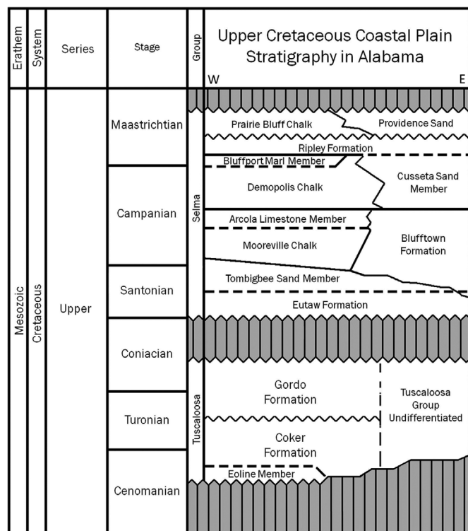
Figure 2. Correlation chart of Upper Cretaceous surface stratigraphy. Light gray areas represent unconformities.
