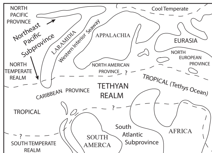
Figure 2. Location of the NEP region, from a portion of Kauffman's (1973:fig. 1) Cretaceous global paleobiogeographic provinces map.
