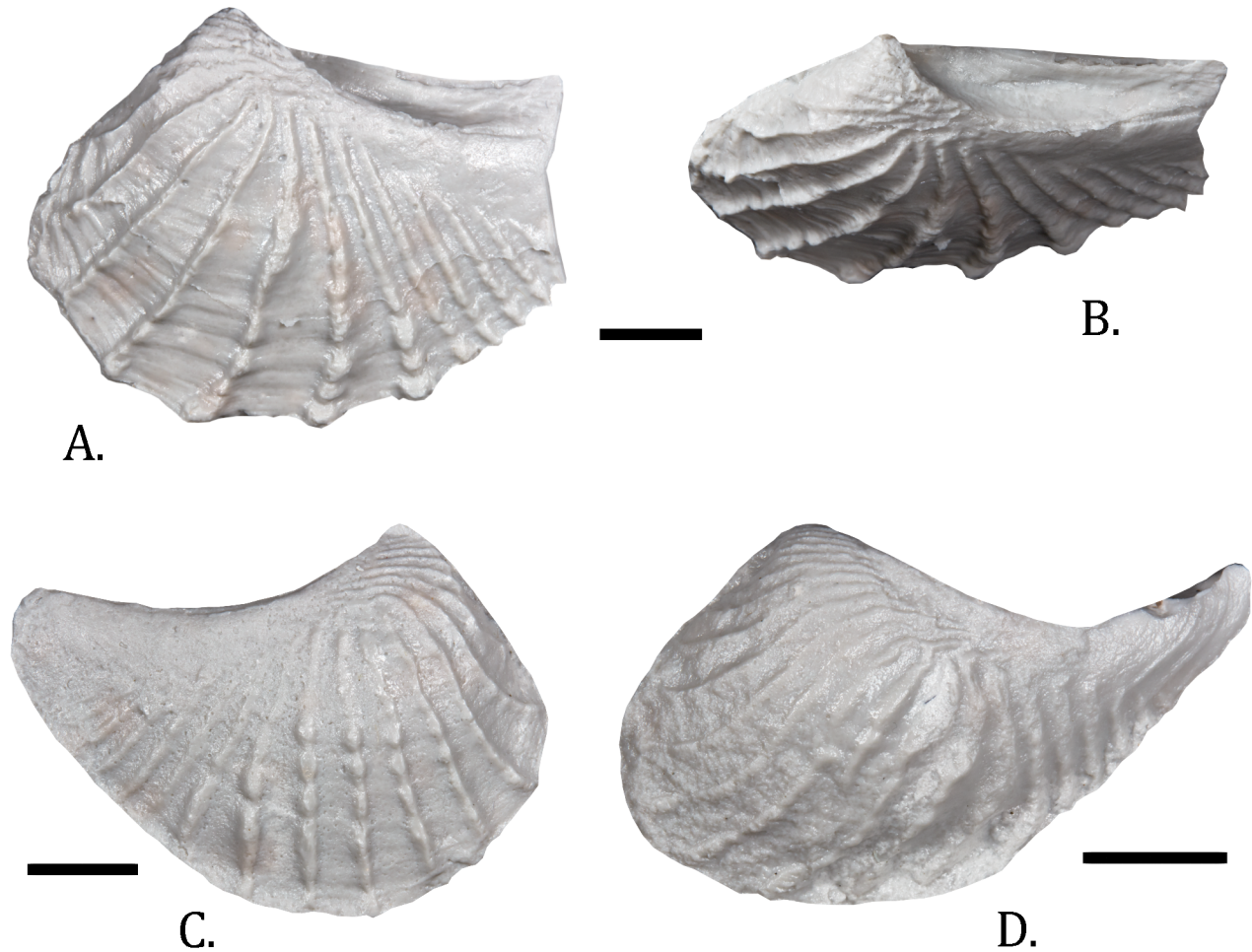
Figure 6. Columbitrignonia condoni (Packard, 1921). All are silicone casts of external molds. A, B. UWBM 112552 from UWBM loc. 9486. Posterior end missing. A. Flank view of LV. B. Oblique view showing area and marginal carina. C. UWBM 112554 from UWBM loc. 9487. Flank view of RV. D. UWBM 112555 from UWBM loc. 9487. Flank view of LV showing commarginal lirae on the posterior terminus. Scale bars = 10 mm.
