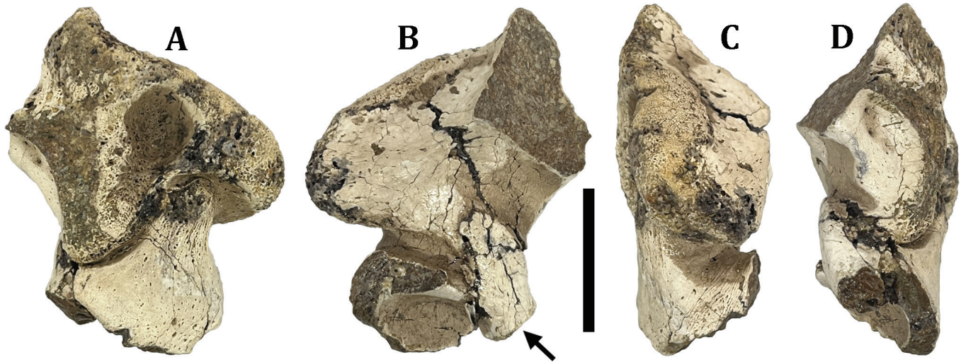
Figure 12: Ectenosaurus shannoni sp. nov., ALMNH:Paleo:5452. A–D. Left quadrate fragment with suprastapedial-infrastapedial contact in posterior (A), anterior/interior (B), lateral (C), and medial (D) views. Arrow indicates interior flange of infrastapedial process. Scale bar=2 cm.
