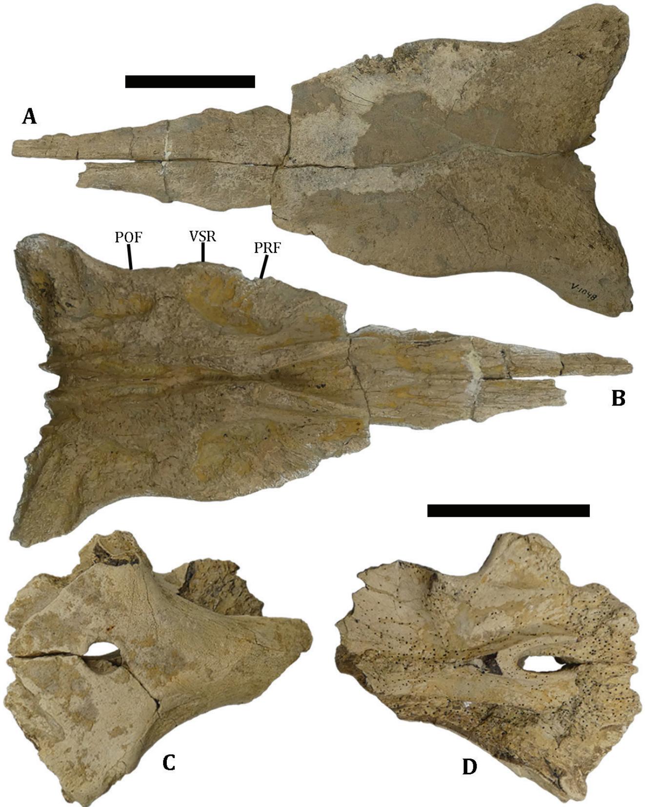
Figure 11. Ectenosaurus shannoni sp. nov., ALMNH:Paleo:5452. A, B. Frontal in dorsal (A) and ventral (B) views. C, D. Parietal in dorsal (C) and ventral (D) views. Abbreviations: POF, excavation for postorbitofrontal; PRF, excavation for prefrontal; VSR, ventral separation ridge. Scale bars=5 cm.
