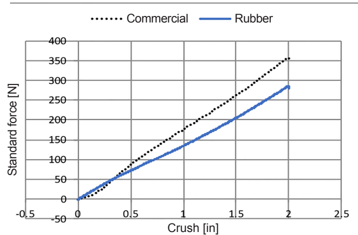
Figure 5. Tensile test results of simulated chest compression.
