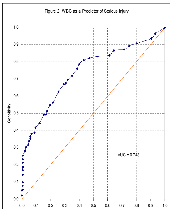
Figure 2. WBC as a Predictor of Serious Injury
