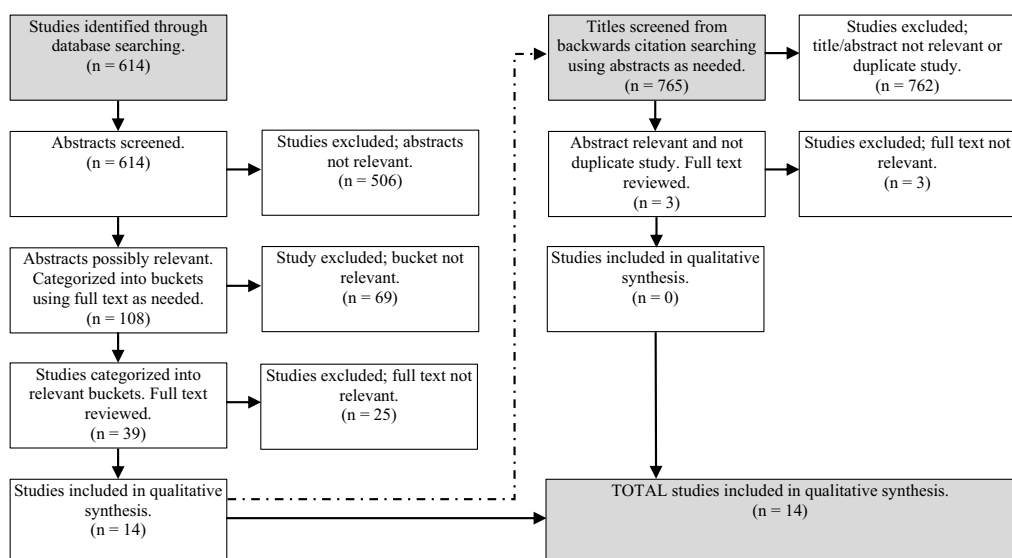
Figure 1. PRISMA flowchart.
