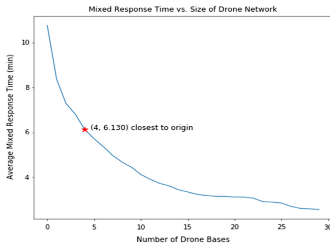
Figure 3. Average response time given number of drone bases. This figure demonstrates the relationship between the number of drone bases and response time. The red star represents the point closest to the origin (x-axis must be a whole number). This point corresponds to the most efficient use of drone resources.
