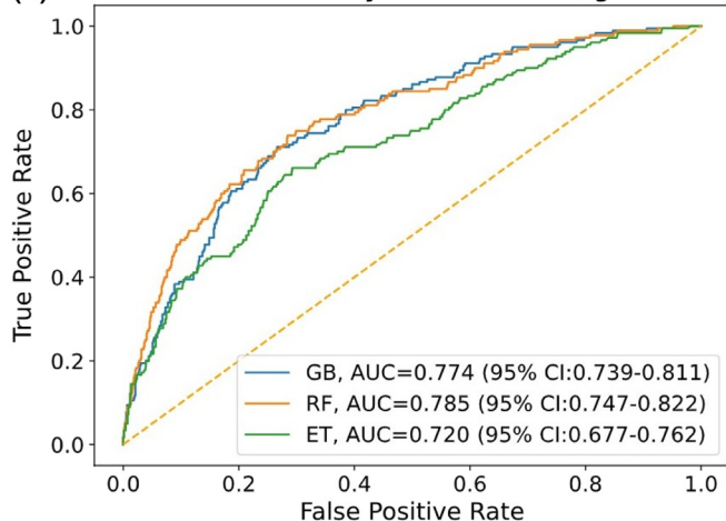
(A) ROC Curve Analysis for the Testing Set
