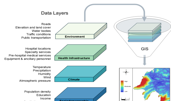
Figure 1. Various data layers can be combined in geographic information systems software to visualize climate hazard risk of a study area.
