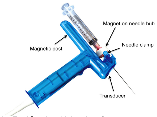
Figure 2. AxoTrack® probe with location of sensors.
